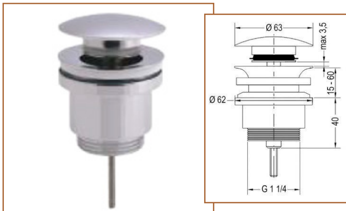
VALVULA CLIC CLAC CROMADA L173964 M50 12,95 €
